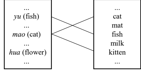
Figure 1: Illustration of the target-to-source matching for the Chinese-English language pair. Each target word in the corpus (right) is matched to a single source word (left). Target words shown without a link (“mat” and “milk”) are implicitly matched to the special empty source word.
